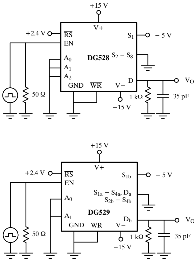
Figure 6. Enable t_{ON}/t_{OFF} Time
