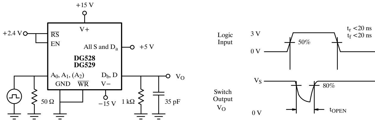
Figure 4. Break-Before-Make
