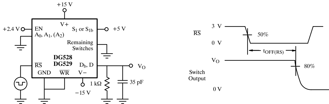
Figure 8. Reset Turn-Off Time t_{OFF(RS)}
